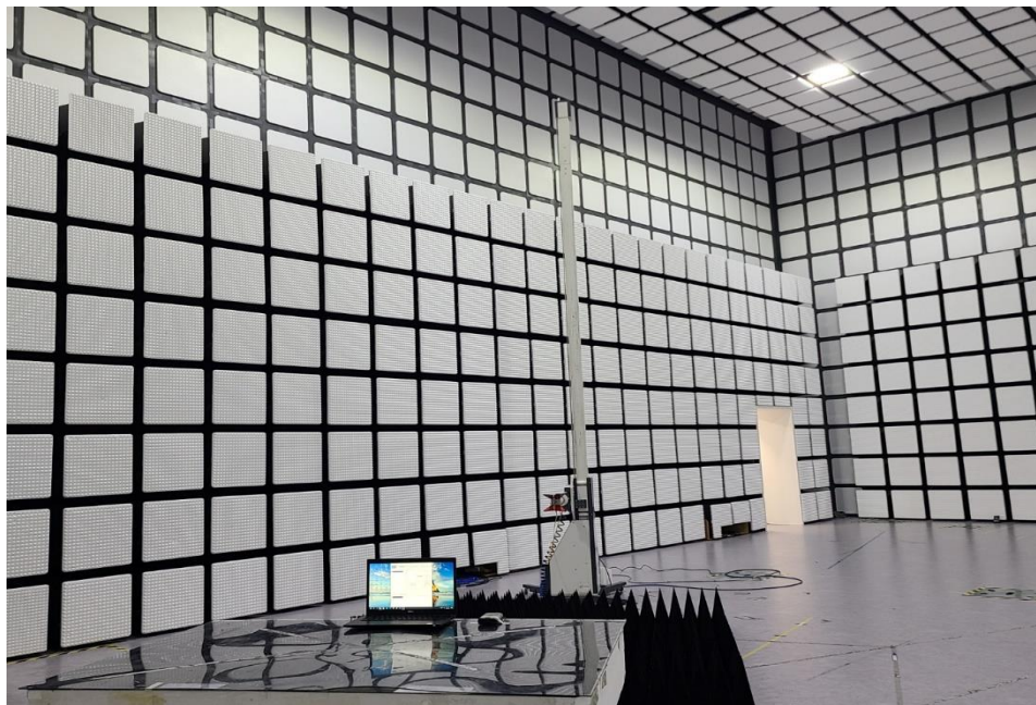
Radiated Emission (1 GHz ~ 6 GHz)
