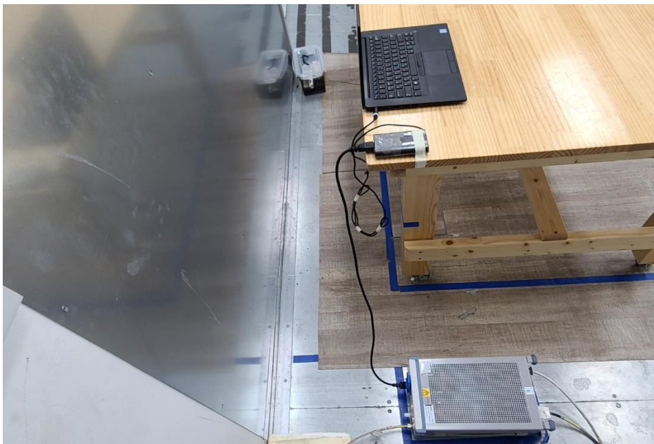
Conducted Emission
