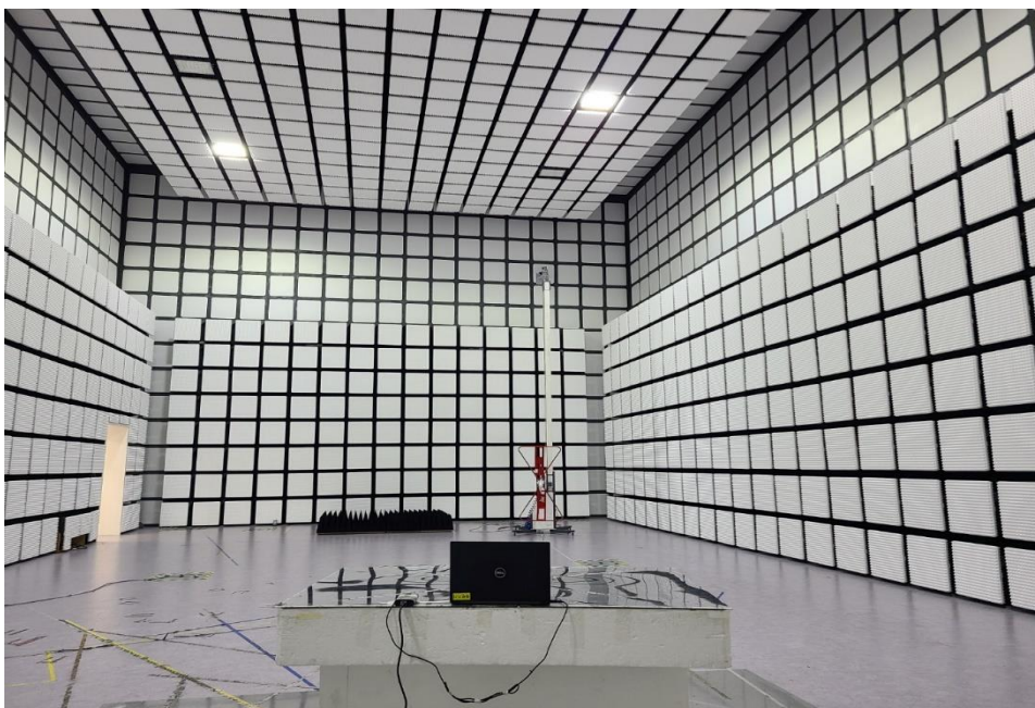
Radiated Emission (30 MHz ~ 1 GHz)
